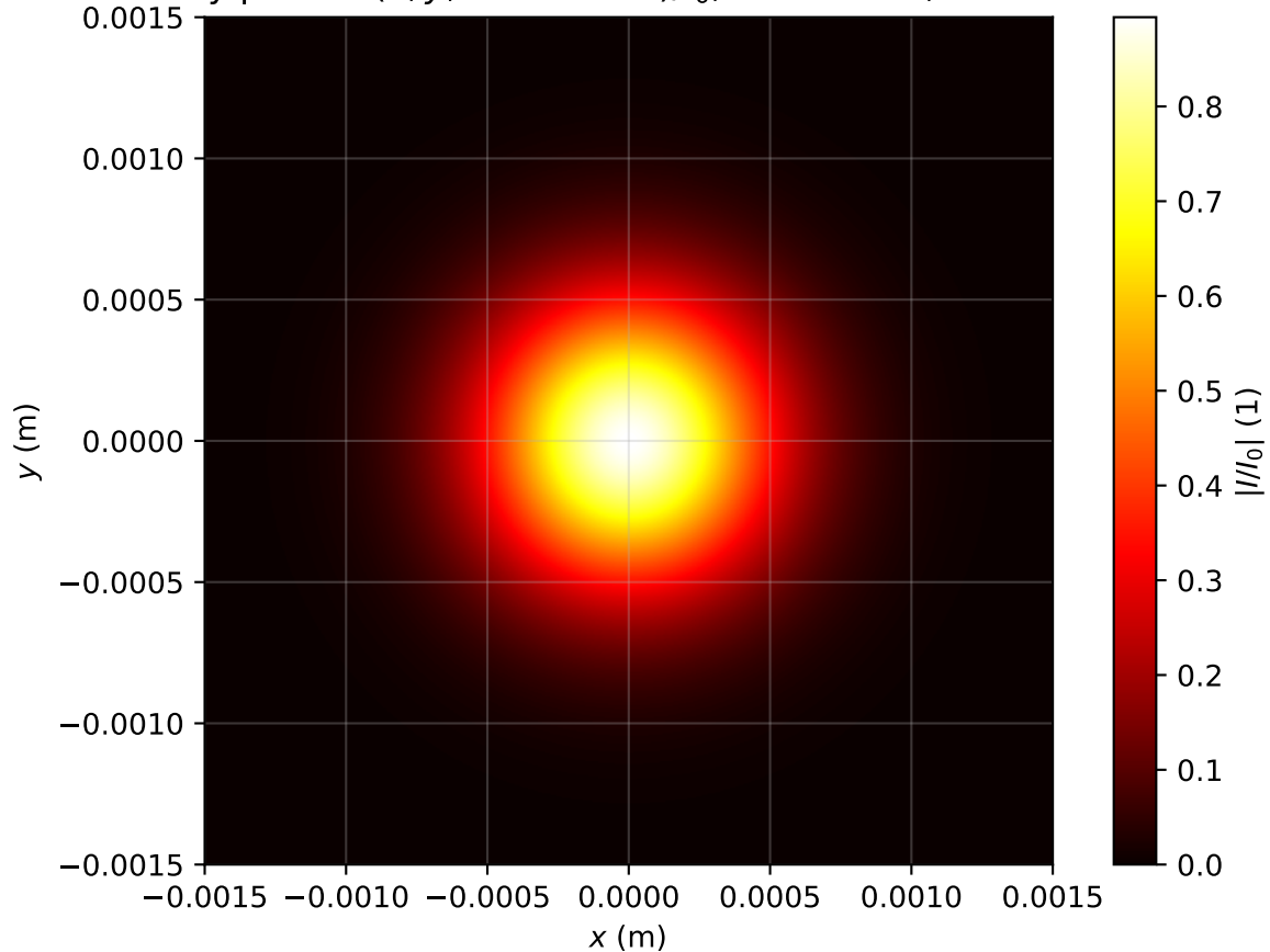
Intensity profile I(x, y, z = 0.955m)/I_0 , \text{Pin}=0.2\text{Pcr} , artificial time
